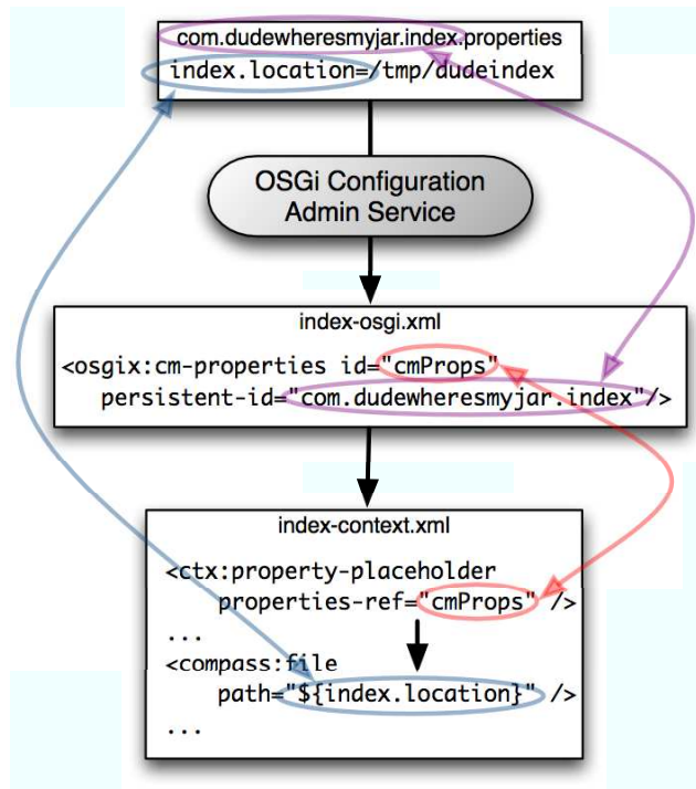
Figure 10.2: Spring-DM's <osgix:cm-properties> pulls configuration details from the OSGi Configuration Admin Service and makes it available to Spring's property placeholder facility.
