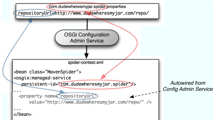
Figure 10.3: Spring-DM's <osgi:managed-service> autowires a bean's properties with values pulled from the OSGi Configuration Admin Service.
